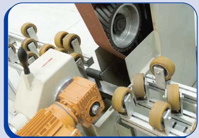
Guide Wheel
